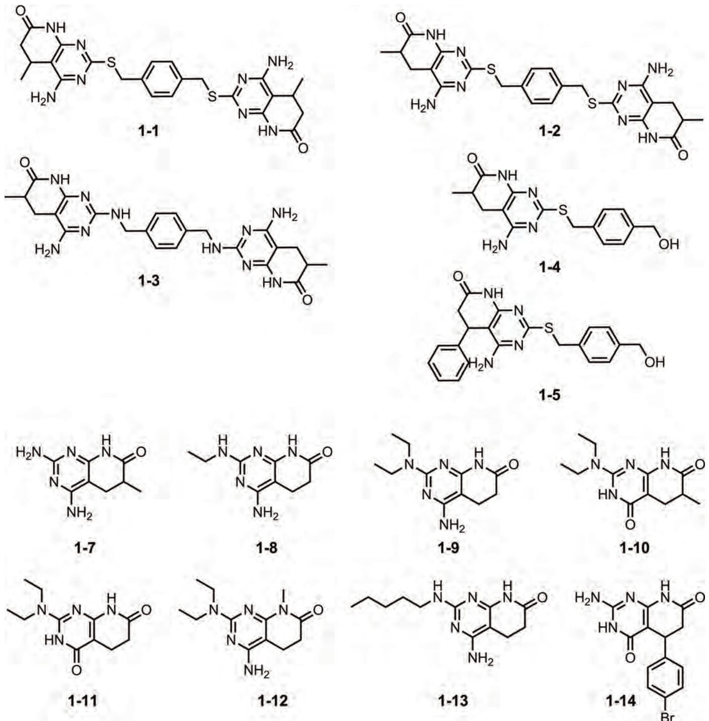
Fig 3. The molecular structure of the compounds we considered, based on the pyrido[2,3-d]pyrimidine scaffold (compound family 1). This family is divided into dimers (1-1 to 1-3) and monomers (1-4 to 1-14).
