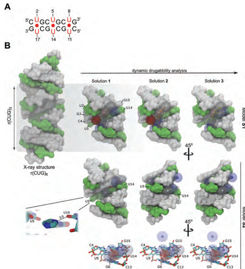
Fig 5. (A) Schematic representation of the r(CUG) 3 model system. (B) Druggability analysis description of the S1 and S2 model systems. RNA is shown as a surface representation with C•G and G•C pairs in white and U-U pairs in green; three druggability solutions were obtained per system. Each druggable region, or hotspot, is represented by a colored sphere (red to blue, from lowest to highest binding-energy, respectively). Notice that the druggable sites in model S1 are distributed along the major groove but are mainly located in the U-U pairs. Model S2 had a stacking interaction pattern caused by the imidazole fragment, which stacks via one U-U pair and forms an H-bond with the O4 atom of U14 (3.0 Å). Some features can also be observed along the minor groove.
