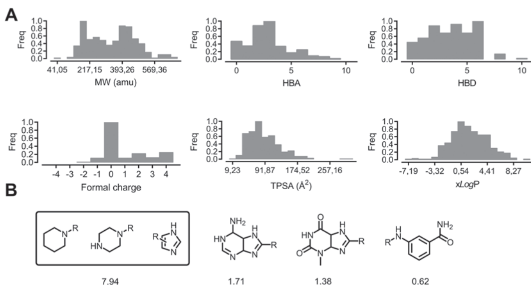
Fig 2. (A) Distribution of the principal physicochemical properties in our in-house chemical library containing more than 300 compounds: molecular weight (MW), hydrogen bond acceptors (HBAs), hydrogen bond donors (HBDs), formal charge, topological surface area (TPSA), and xlogP . (B) The most commonly observed fragments were ordered by their activity-adjusted frequency values (see Methods for a detailed description).
