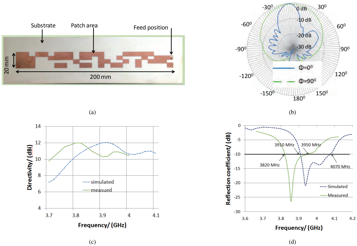
Fig. 10. Fabrication results of the optimized patch. (a) Photo of the antenna. (b) Normalized measured main radiation cuts at 3820 MHz ( \phi=0^\circ corresponds to the E plane). (c) Directivity vs. frequency. (d) S11 plots.
