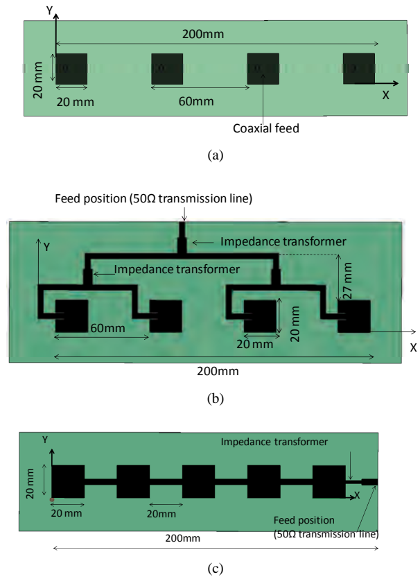
Fig. 1. Antenna configurations: (a) Coaxial-fed antenna array. (b) Corporate-fed microstrip array. (c) Series-fed microstrip array.
