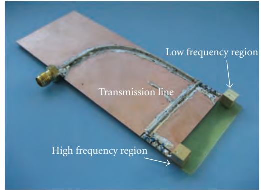
FIGURE 33: Pentaband prototype designed including the reactance cancellation inductor, the broadband matching network, and the notch filters required for providing isolation between both frequency regions.
