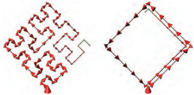
FIGURE 13: Current vector distribution of the antennas at the resonance frequency of f = 84.5 MHz.
