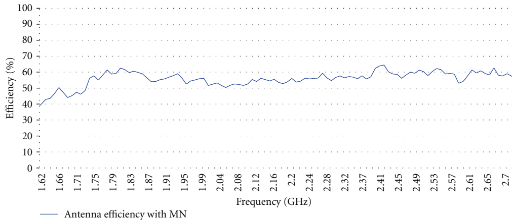
FIGURE 23: Measured antenna efficiency of the L-monopole shown in Figure 22. Broadband matching network consisting of a shunt L = 3.3 nH and a shunt C = 1.3 pF.
