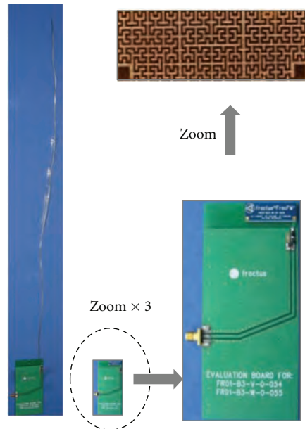
FIGURE 10: External wire (75 cm length) and internal FM Chip Hilbert antennas (30 mm × 10 mm) integrated within a typical smartphone platform [19–21].
