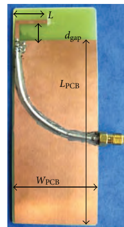
FIGURE 22: L-shaped monopole printed on a ground plane. The dimensions of the monopole antenna are L = 23 mm with a strip width of 2 mm, and it is located in the shorter edge of a PCB at a distance D_{\text{gap}} = 4 mm from the ground plane. The PCB dimensions are L_{\text{PCB}} = 90 mm and W_{\text{PCB}} = 40 mm.
