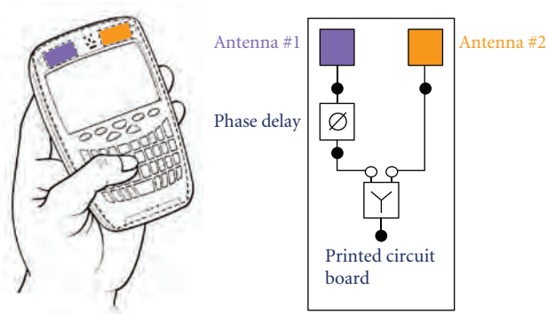
FIGURE 18: Illustration of a distributed antenna system having two elements placed at different locations of a handset device.
