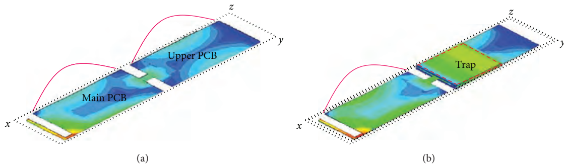
FIGURE 29: Simulated current distribution at 1.82 GHz without and with a shortening mechanism consisting of a short circuit plate of \lambda/4 at 1.82 GHz. The continuous line is a qualitative approach of the currents on the ground plane. For (a), a current mode having two sinusoids is supported causing a multi-lobe pattern. For (b), the current in the upper PCB board has been mitigated due to the trap.
