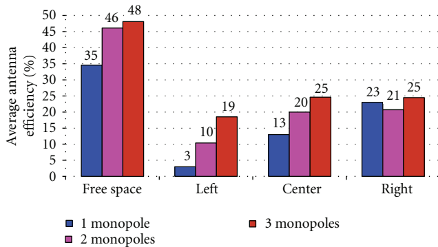
FIGURE 21: Comparisons of the measured average antenna efficiency (824–960 MHz) in free space and regarding hand loading for the proposed antenna systems depicted in Figure 19 and regarding the three positions of the finger.
