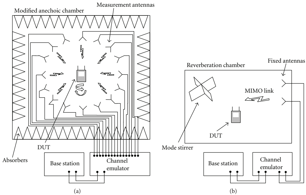
FIGURE 9: Example measurement setups for active MIMO testing of antennas for wireless handheld devices.
