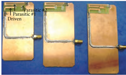
FIGURE 16: Prototypes regarding a ground plane of 45 mm \times 90 mm, 100 mm, and 110 mm. The driven element is fed through a 50 \Omega transmission line.
