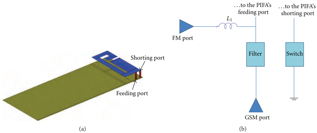
FIGURE 11: (a) 3D view of the PIFA. Ground plane size is 100 mm × 40 mm and PIFA is 38 mm × 15 mm × 6 mm; (b) proposed matching network including a switching circuit, a filter, and a series inductor.
