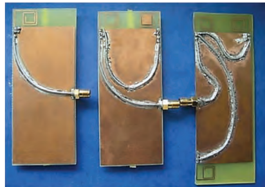
FIGURE 19: Single monopole (left); an array of two monopoles (middle); an array of three monopoles (right). Ground plane is 90 mm \times 40 mm printed on an FR4 substrate 1 mm thick. Monopoles are 13 mm \times 11 mm.
