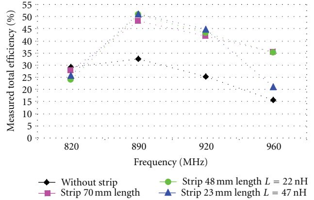
FIGURE 28: Measured total efficiency without the strip and with the strip considering loading inductors for the case shown in Figure 27. The case having L of 22 nH and 48 mm length effectively enhances the efficiency across the 820–960 MHz band.
