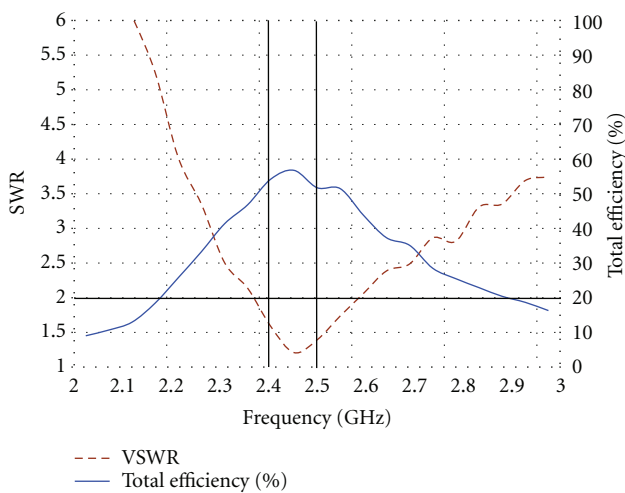
FIGURE 15: Measured SWR and total efficiency for the 2.4-2.5 GHz antenna shown in Figure 14.
