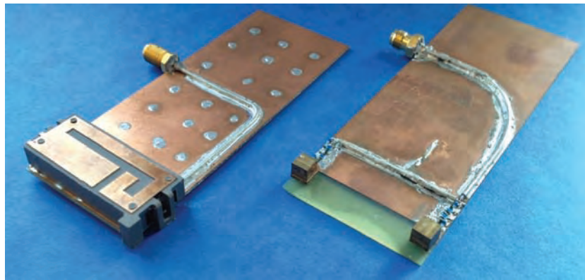
FIGURE 30: Comparison of a PIFA antenna and the solution based on ground plane boosters for operation at GSM850/900, DCS, PCS, and UMTS. The volume of the PIFA is 4600 \text{ mm}^3 , whereas the compact solution is only 250 \text{ mm}^3 .
