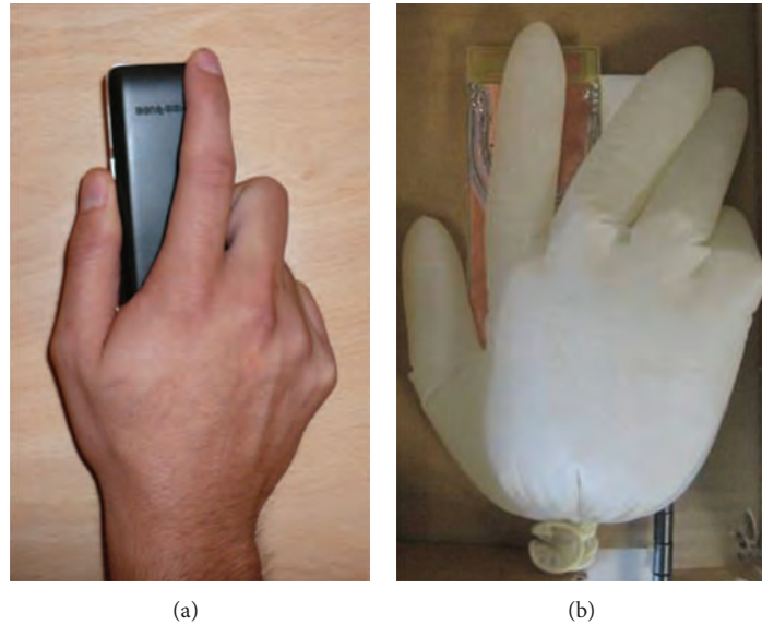
FIGURE 20: (a) Common holding position during a call; (b) the hand phantom emulating the real situation illustrated in (a).
