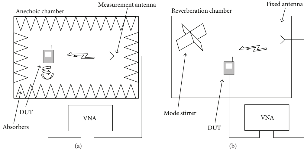
FIGURE 8: Example measurement setups for passive (cable-fed) testing of antennas for wireless handheld devices. For active device testing the DUT is replaced by a functional handset, and the vector network analyzer (VNA) is replaced by a base station simulator.
