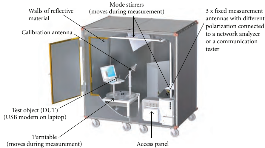
FIGURE 7: Reverberation chamber configured for measurements of antennas for wireless handheld devices.
