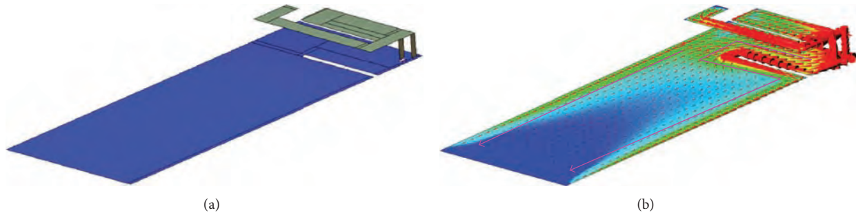
FIGURE 24: (a) Introducing slots in the ground plane to electrically lengthen the current path. (b) Continuous arrows are a qualitative representation of the main current distribution for 900 MHz which is distributed along the long edges of the PCB. PCB is 100 mm × 40 mm.
