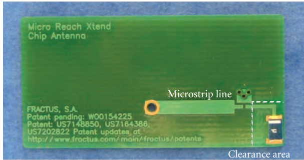
FIGURE 14: SMD space-filling-based antenna for 2.4-2.5 GHz applications. Antenna is 4.1 \text{ mm} \times 2 \text{ mm} \times 1 \text{ mm} ( 4.1 \text{ mm} is 0.033\lambda at 2.45 \text{ GHz} ).
