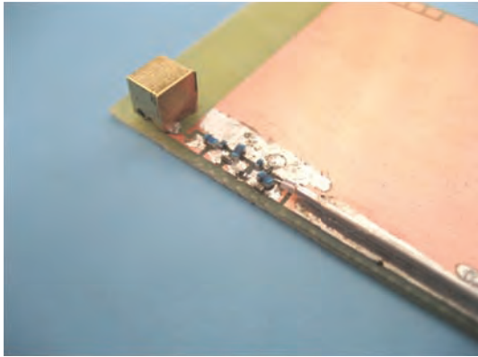
FIGURE 32: Single-band prototype including the reactance cancellation inductor and the broadband matching network.
