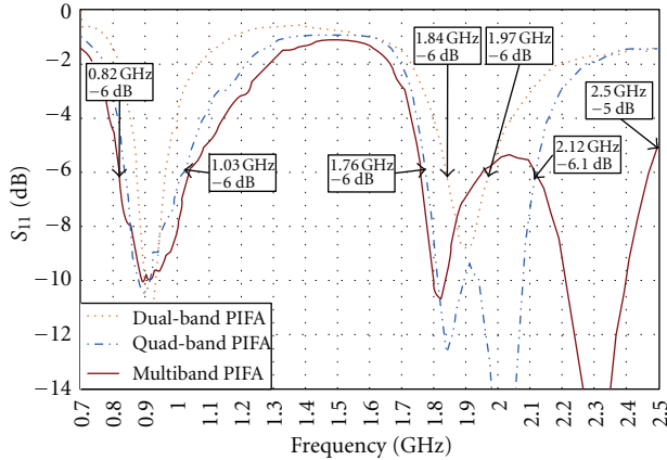
FIGURE 26: Measured reflection coefficient for the three studied prototypes. It can be seen how the proposed multiband design can operate at least over the GSM850, GSM900, DCS, PCS, UMTS, and Bluetooth bands.
