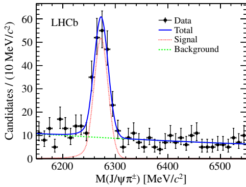
FIG. 2 (color online). Invariant mass distribution of B_c^+ \rightarrow J/\psi \pi^+ decays, used in the mass measurement. The fit to the data is superimposed.
