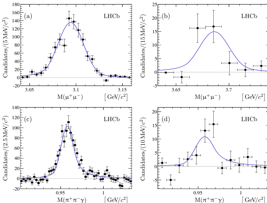
Figure 6. Background subtracted \psi \rightarrow \mu^+\mu^- (a, b) and \eta' \rightarrow \pi^+\pi^-\gamma (c, d) mass distributions in B_s^0 \rightarrow \psi\eta' decays. The figures (a, c) correspond to the J/\psi channel, and the figures (b, d) correspond to the \psi(2S) channel. The solid curves represent the total fit functions.
