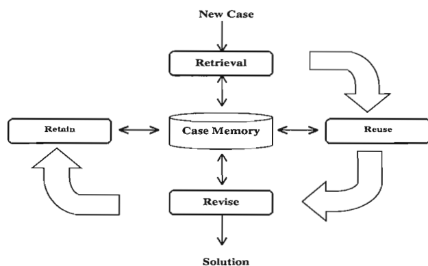
Figure 1: CBR Cycle.
