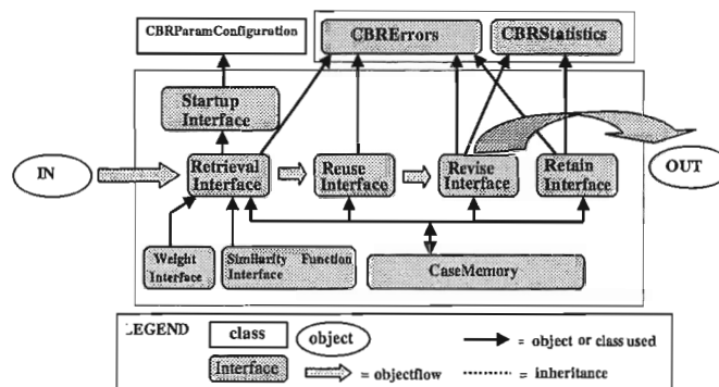
Figure 2: General Structure in BASTIAN.
