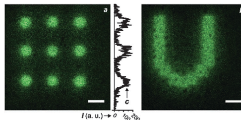
Fig. 6 Confocal laser-scanning fluorescence images (a and b, \lambda_{\text{Ex}} = 405 nm, \lambda_{\text{Em}} = 430\text{--}650 nm, scale bar = 30\ \mu\text{m} ) of PBMA films, doped with 1 (3% w/w) and deposited on glass slides with silver nanoparticles on their surface, recorded after illumination ( \lambda_{\text{Ac}} = 405 nm, 0.1 mW, 300 s) of defined areas within the imaging field. Profile of the emission intensity (c) measured across some of the activated areas in a.
