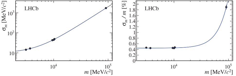
Fig. 19. Mass resolution ( \sigma_m ) (left) and relative mass resolution (right) as a function of the mass ( m ) of the dimuon resonance. The mass of the muons can be neglected in the invariant mass calculation of these resonances. The mass resolution is obtained from a fit to the mass distributions. The superimposed curve is obtained from an empirical power-law fit through the data points.
