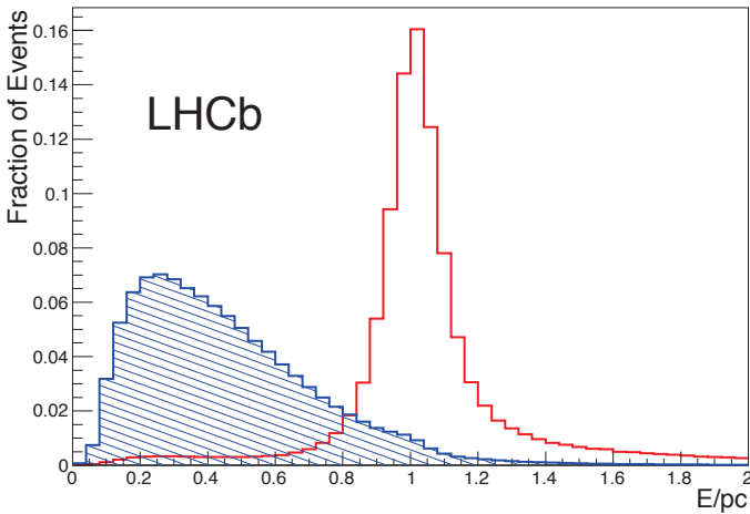
Fig. 34. Distribution for the ECAL of E/pc for electrons (red) and hadrons (blue), as obtained from the first 340 \text{ pb}^{-1} recorded in 2011.
