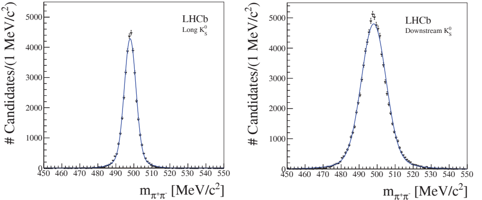
Fig. 27. Distribution of the invariant mass of K_S^0 \rightarrow \pi^+ \pi^- candidates with a decay vertex at a significant distance to the PV, for long tracks (left) and downstream tracks (right). A mass resolution of 3.5 \text{ MeV}/c^2 is achieved for the candidates reconstructed from long tracks and 7 \text{ MeV}/c^2 for those using downstream tracks.
