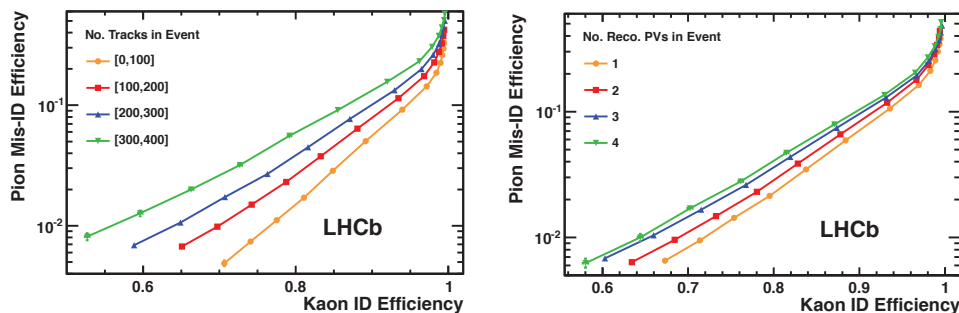
Fig. 40. Pion misidentification fraction versus kaon identification efficiency as measured in 7 TeV LHCb collisions: (left) as a function of track multiplicity, and (right) as a function of the number of reconstructed primary vertices. 82 The efficiencies are averaged over all particle momenta.
