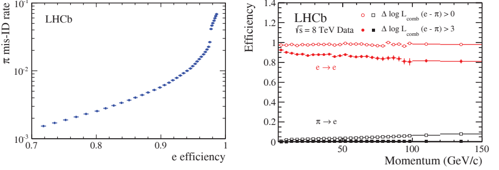
Fig. 42. Electron identification performance using the \Delta \log \mathcal{L}_{\text{comb}}(e-\pi) variable, as measured in 8 TeV collision data, using a tag and probe technique with electrons from the decay B^\pm \rightarrow (J/\psi \rightarrow e^+e^-)K^\pm . Left, pion misidentification rate versus electron identification probability when the cut value is varied. Right, electron identification efficiency and pion misidentification rate as a function of track momentum, for two different cuts on \Delta \log \mathcal{L}_{\text{comb}}(e-\pi) .
